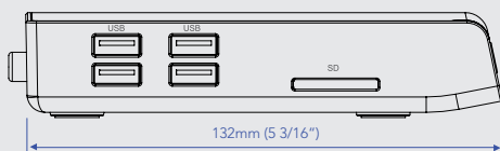
Sideview DSP-H
