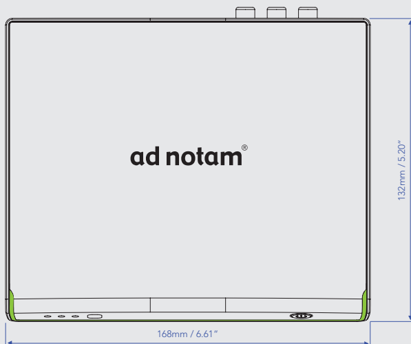
Topview DSP-H
